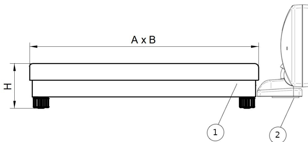
Rys. 3. Wagi WIN-1/1÷WIN-1000/1 wer. D 1-pomost, 2-miernik
